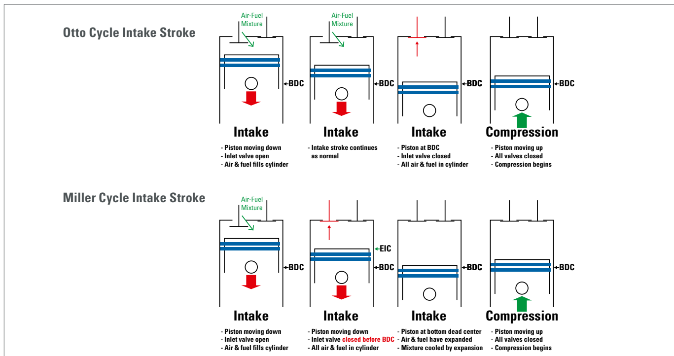
Figure 7: Intake stroke for an Otto Cycle engine (top) and a Miller Cycle engine (bottom)
