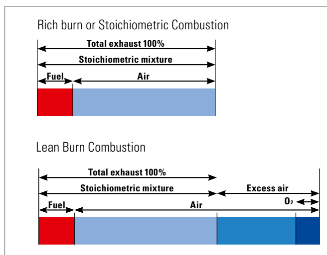
Figure 11: Rich burn (stoichiometric) combustion air/fuel ratio (top) vs. Lean burn combustion air/fuel ratio (bottom)
