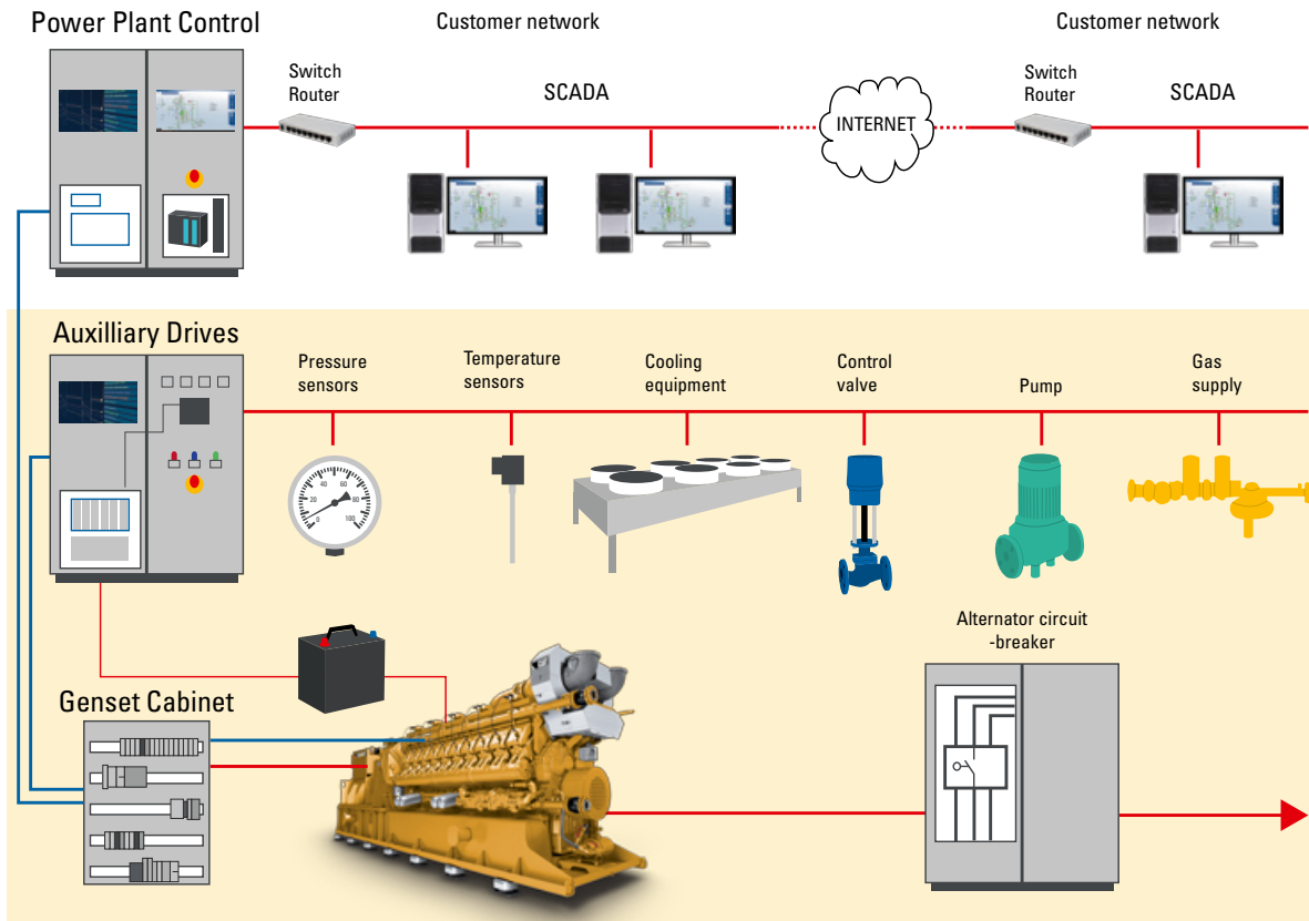
Figure 1: Schematic of a comprehensive gas power plant control system
